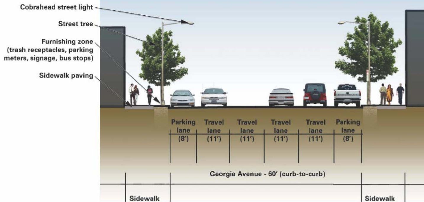
TYPICAL SECTION: EXISTING CONDITIONS
