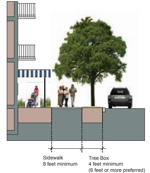
Typical Residential Cross-Section (High Density Residential)
